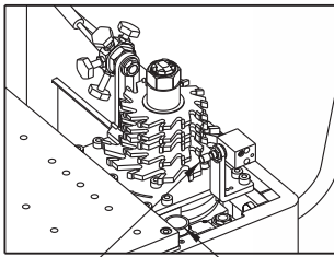
Lubrication cod.502308
